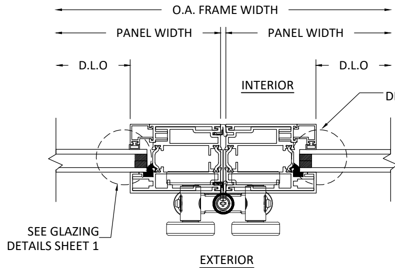
A 5 HORIZONTAL SECTION STILE WITH INTERMEDIATE CARRIER SET DETAIL
