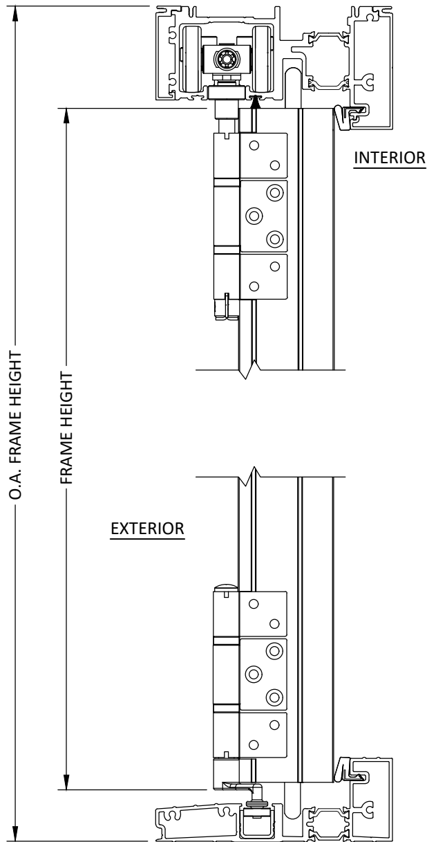
VERTICAL SECTION HEAD AND SILL DETAIL WITH ROLLER WHEELS
