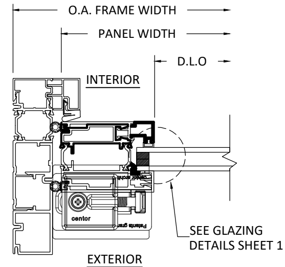
C 5 HORIZONTAL SECTION JAMB WITH PIVOT SET DETAIL
