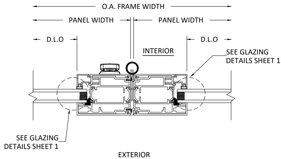
A 5 HORIZONTAL SECTION STILE WITH INTERMEDIATE CARRIER SET DETAIL
