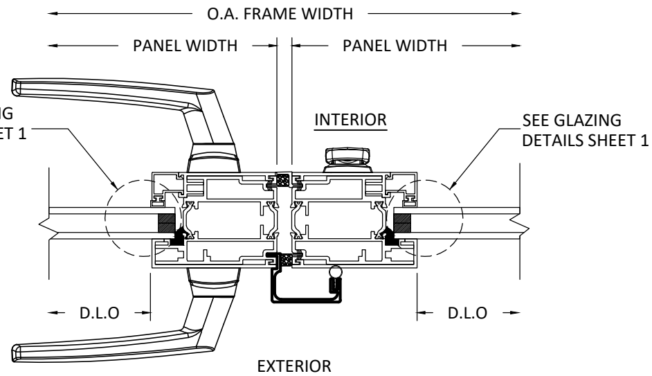
B 5 HORIZONTAL SECTION DOOR HANDLE DETAIL
